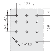
3Z Installation hole position
