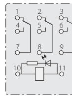
3Z Bottom wiring diagram (with indicator)
