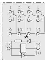
4Z Bottom wiring diagram (with indicator and diode)
