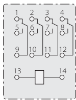
4Z Bottom wiring diagram
