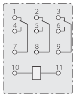
3Z Bottom wiring diagram
