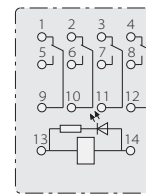
4Z Bottom wiring diagram (with indicator)
