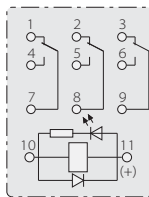
3Z Bottom wiring diagram (with indicator and diode)
